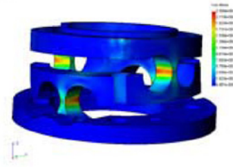
FIGURE 2: FANUC ROBOTICS TAKES FULL ADVANTAGE OF THE SOLID MODELER IN SOLIDWORKS SIMULATION.
