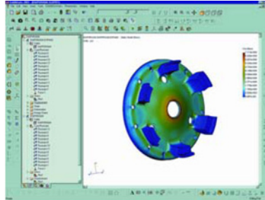
FIGURE 9: CHUCK DESIGNED BY SPEEDGRIP CHUCK INC.
