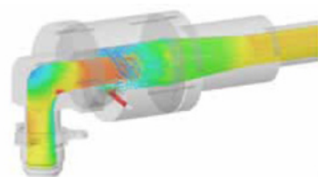
FIGURE 8: CYCLONIC INERTIAL SEPARATOR BY DAVID RACHELS AND HIS ENGINEERING TEAM
