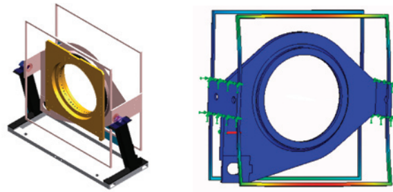
FREQUENCY ANALYSIS ON A SUBASSEMBLY OF A CT SCANNER
